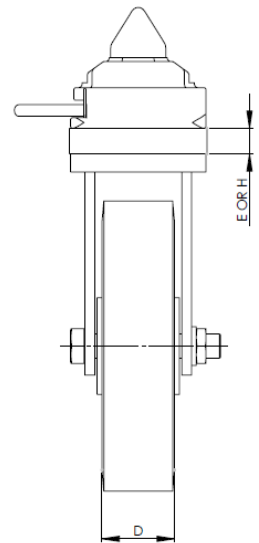
(E) Swivel top plate thickness 26mm
