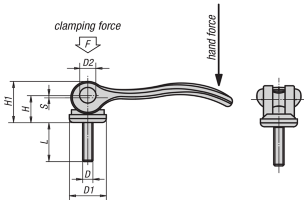
Cam lever with external thread
